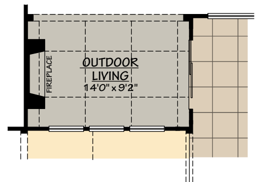
OPT. OUTDOOR LIVING AT FIREPLACE
